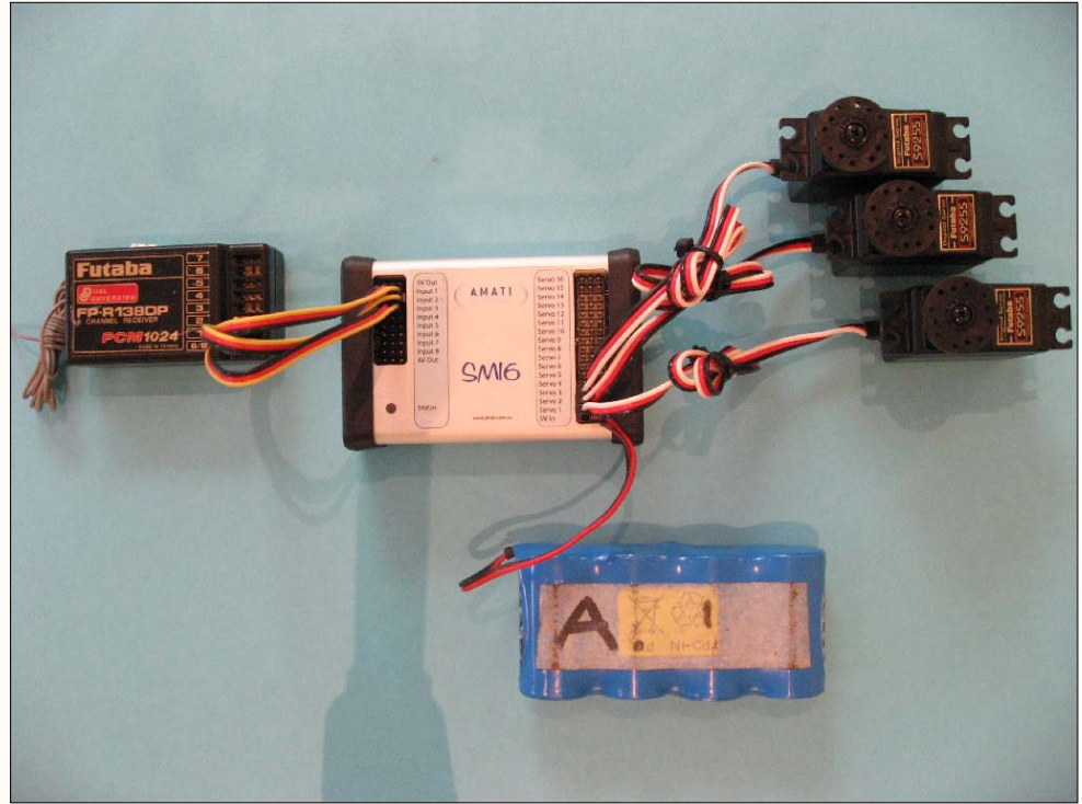
Receiver, SM16, Battery, RC Servos
